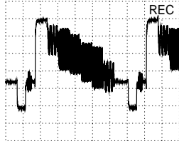
AC, 200mV/Div, 10µs/Div C2881
