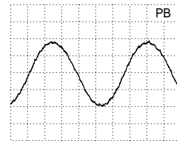
AC, 200mV/Div, 200µs/Div C2652
