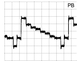
AC, 100mV/Div, 10µs/Div IC7007-(42)
