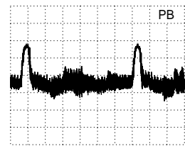
DC, 500mV/Div, 10µs/Div IC7110-(1) ⑥⑤
