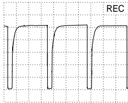
DC, 1V/Div, 20µs/Div IC7800-(17)
