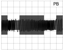
AC, 200mV/Div, 10µs/Div IC7007-(20)
