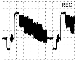
AC, 200mV/Div, 10µs/Div IC7540-(13)
