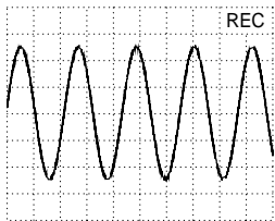
AC, 200mV/Div, 500µs/Div IC7513-(3) / C2503
