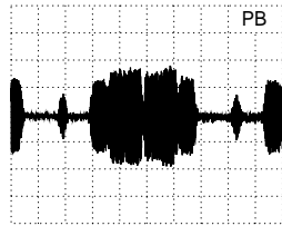
AC, 100mV/Div, 10µs/Div IC7007-(46), PAL
