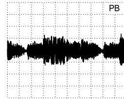
AC, 100mV/Div, 10µs/Div IC7007-(46), SECAM L
