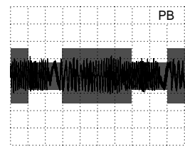
AC, 200mV/Div, 10µs/Div IC7007-(15) ⑦②
