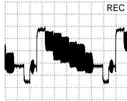
DC, 500mV/Div, 10µs/Div IC7007-(38)
